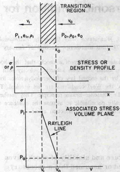
FIG. 1. Shock transition layer, compressive shock.
